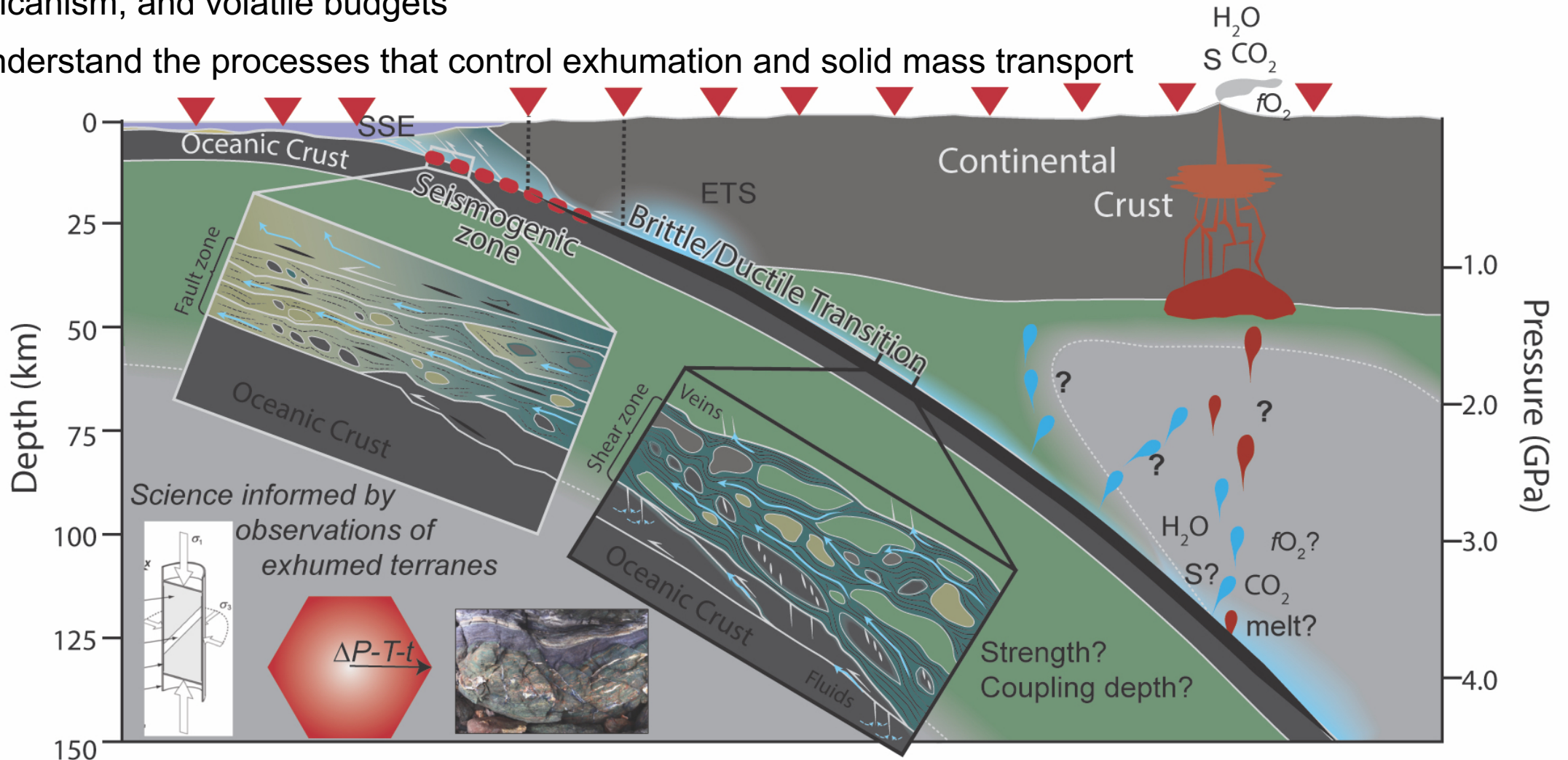
Exhumed rocks, fluid and rheology (groups 3 and 7)
